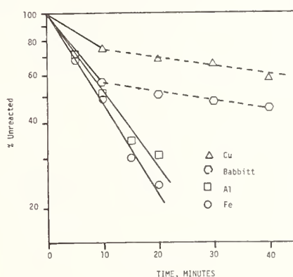
Figure 2. Oxidative degradation of a superrefined mineral oil, PRL7828, on different metals. Microoxidation test conditions include: 40 \mu\text{l} and 225 ^{\circ}\text{C} .
